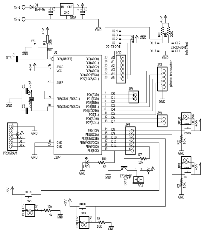
Fig. 5. Microcontroller
